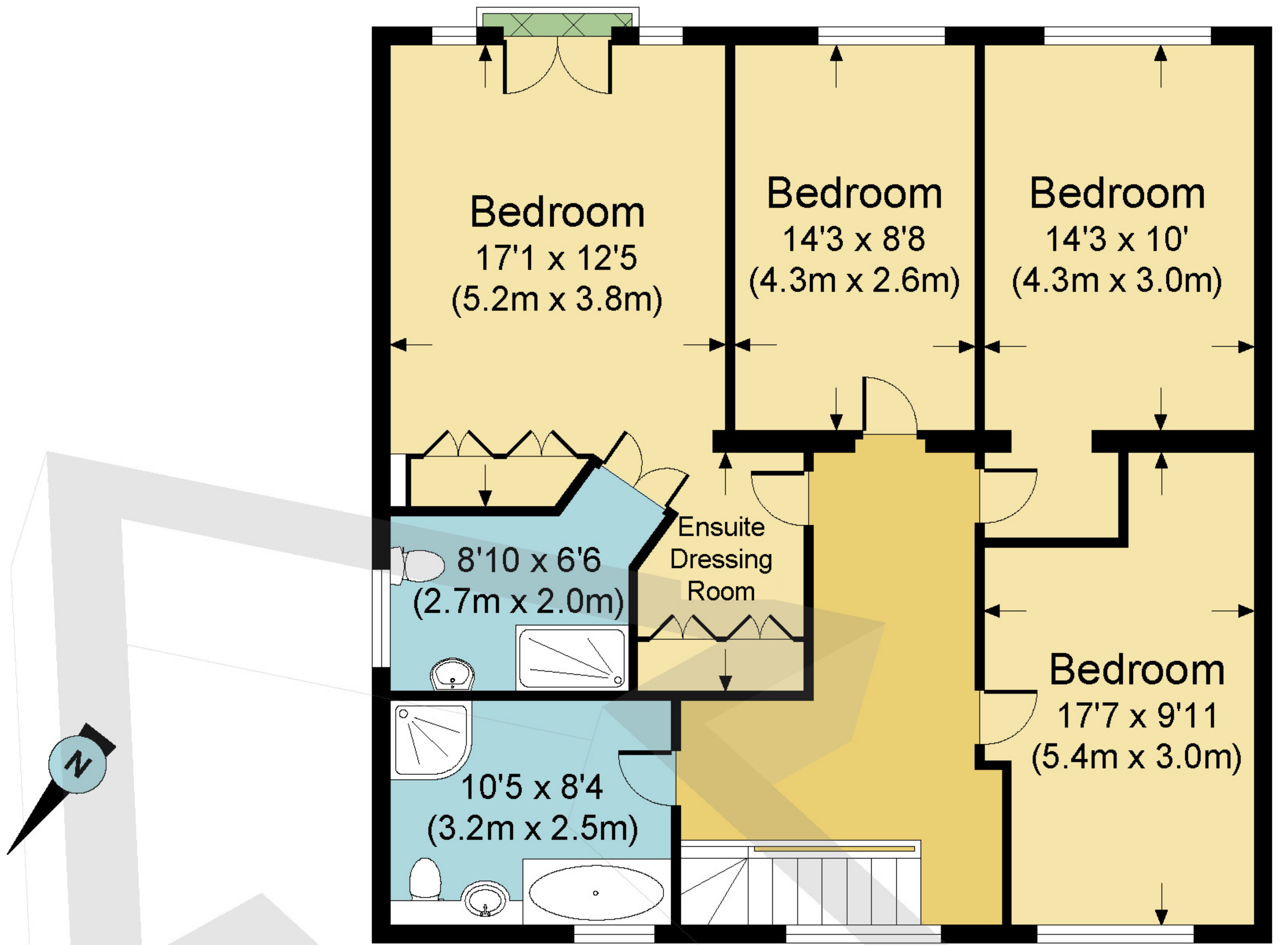
First Floor
