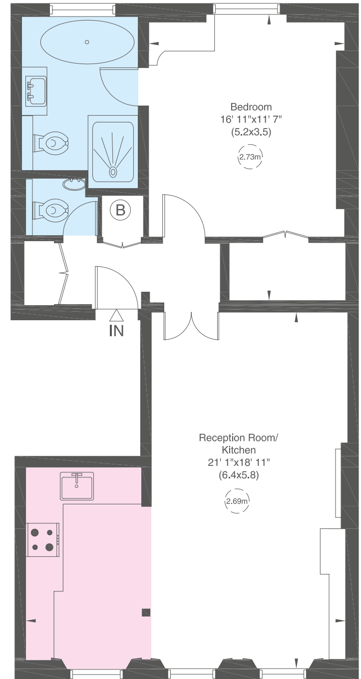
THIRD FLOOR
