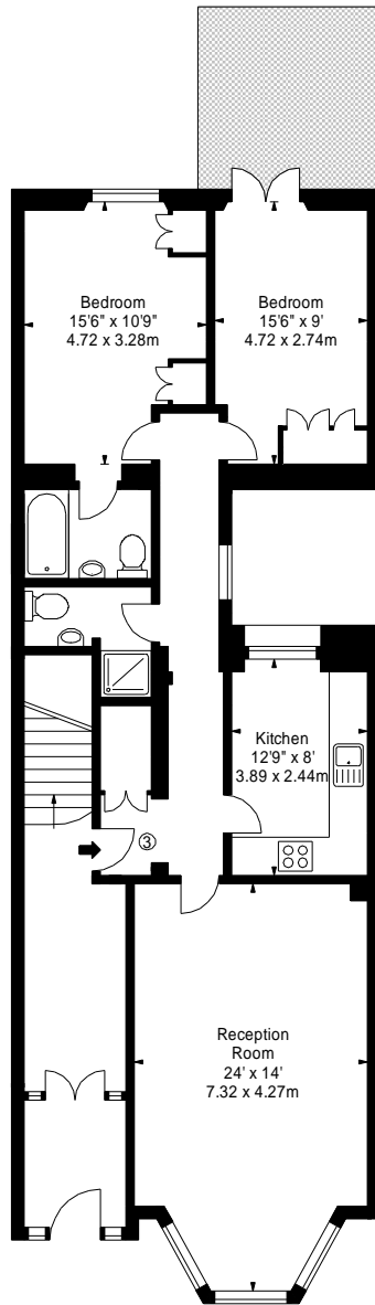
GROUND FLOOR
