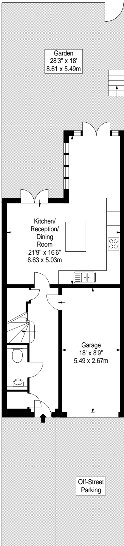
GROUND FLOOR
