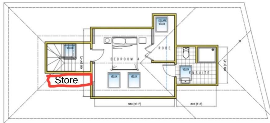
EXISTING ROOFSPACE FLOOR PLAN scale 1:50
