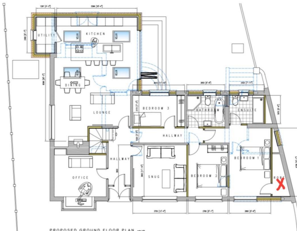
PROPOSED GROUND FLOOR PLAN scale 1:50
