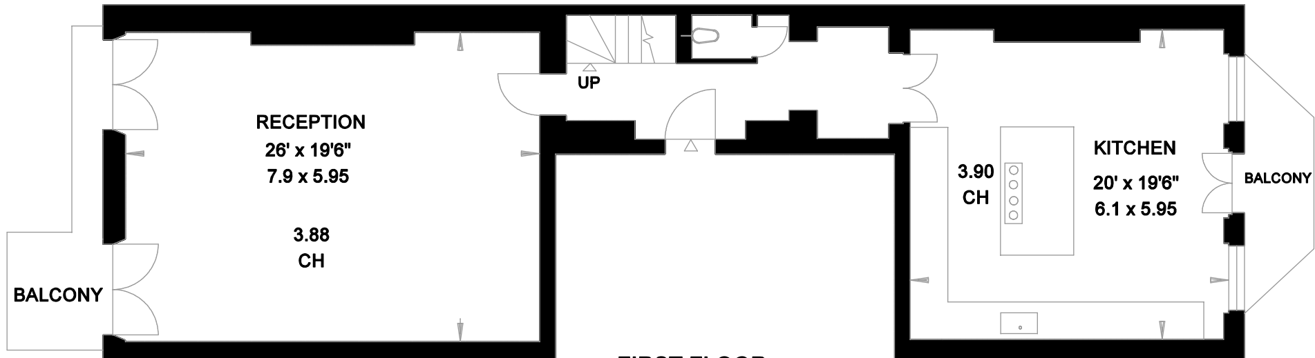
FIRST FLOOR
