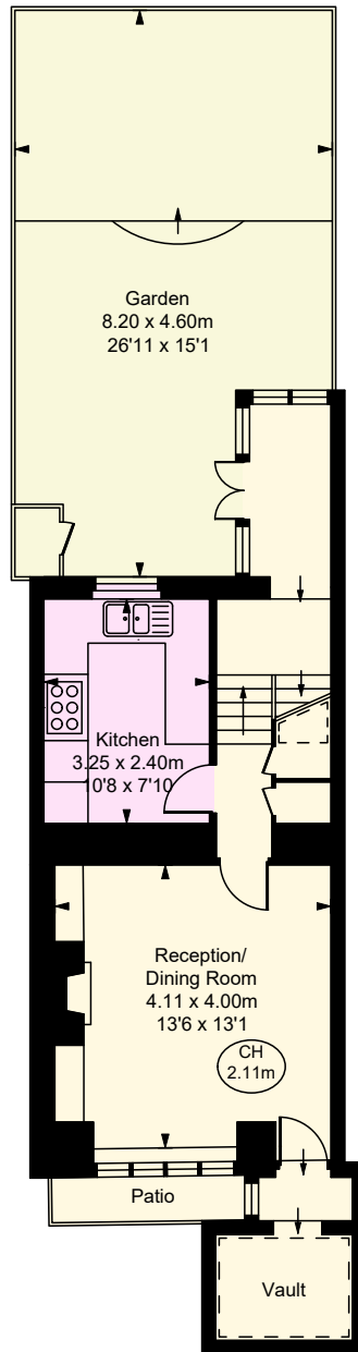
Lower Ground Floor Approximate Gross Internal Area 39.91 sq m / 430 sq ft
