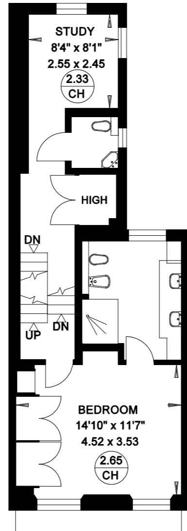
FIRST FLOOR
