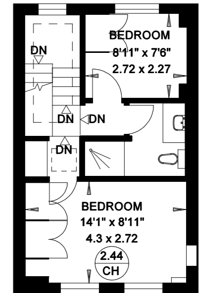
THIRD FLOOR
