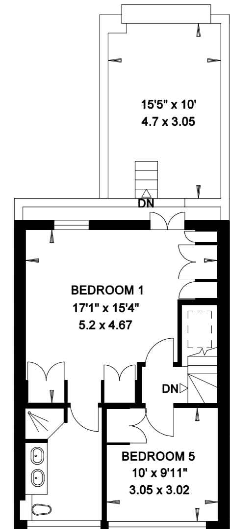
THIRD FLOOR
