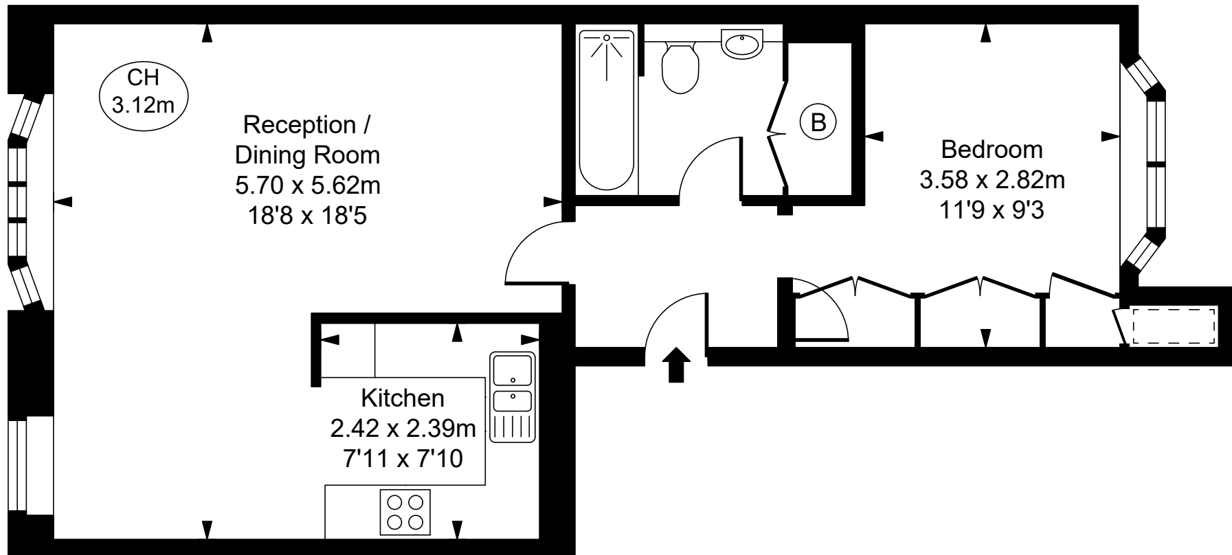
Ground Floor
