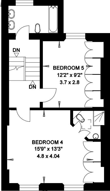
THIRD FLOOR
