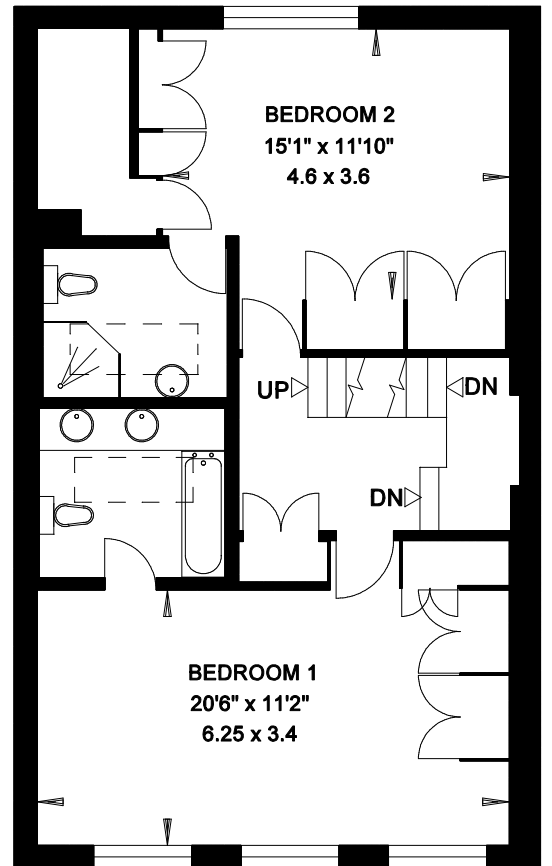
FIFTH FLOOR
