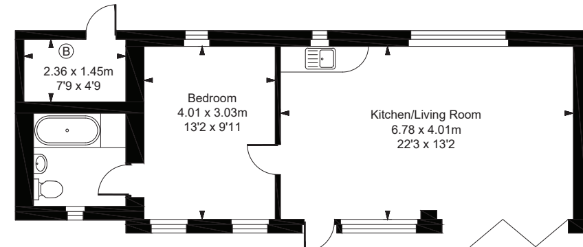
Annexe Approximate Gross Internal Area 49.97 sq m / 538 sq ft
