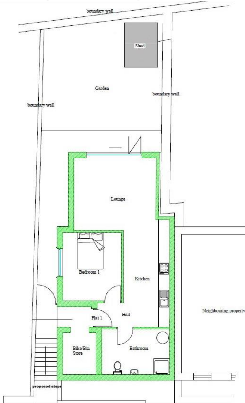
Proposed Basement Floor Layout Plan
