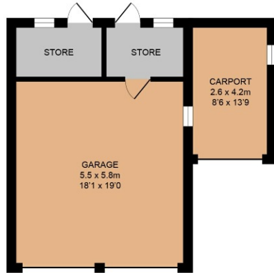
GARAGE & STORE APPROX. FLOOR AREA 53.0 SQ.M. (570 SQ.FT.)
