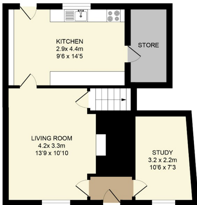
GROUND FLOOR APPROX. FLOOR AREA 43.0 SQ.M. (463 SQ.FT.)
