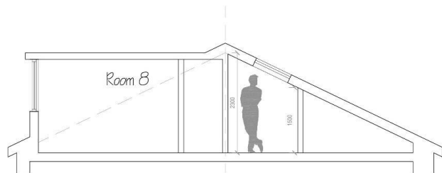
SCHEMATIC SECTION 1:50
