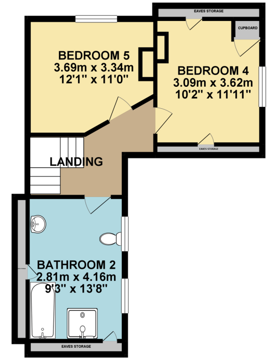
2ND FLOOR 45.55 sq. m. ( 490.30 sq. ft. )
