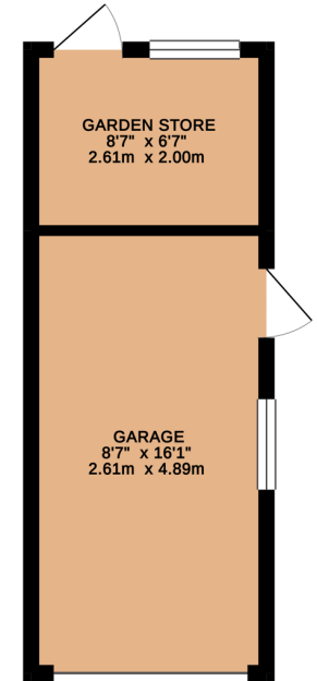
ENTRANCE FLOOR 196 sq. ft. ( 18.2 sq. m. )
