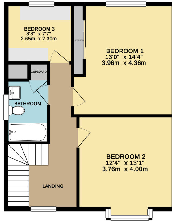
1ST FLOOR 572 sq. ft. ( 53.2 sq. m. )
