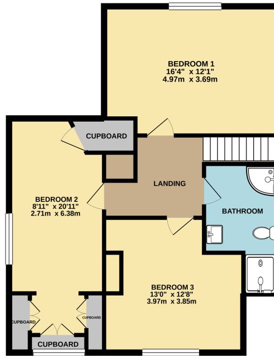
1ST FLOOR 707 sq. ft. (65.6 sq. m.) approx.
