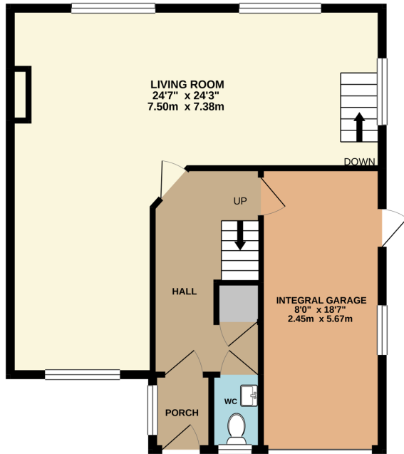
GROUND FLOOR 522 sq.ft. (48.5 sq.m.) approx.
