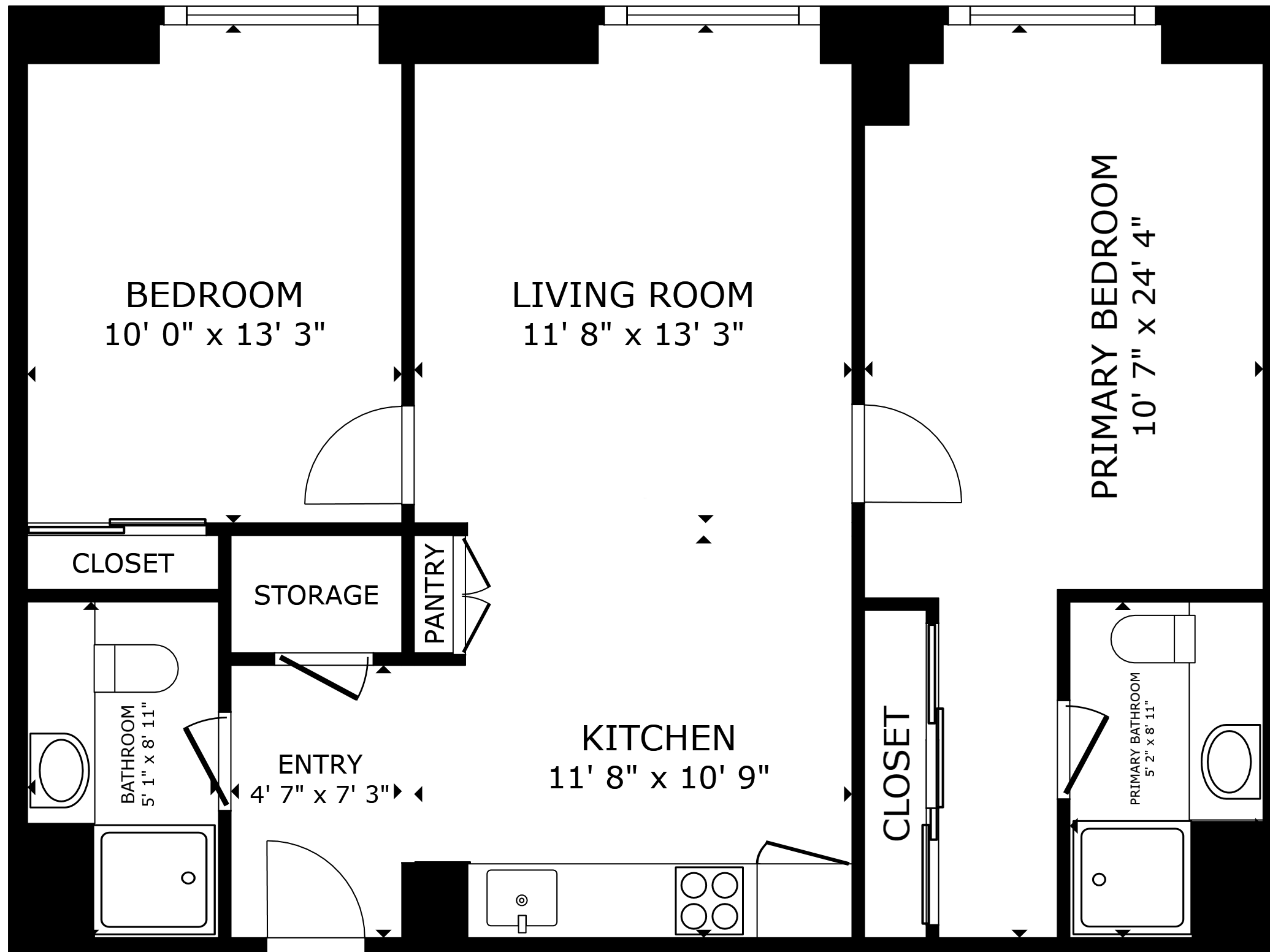
FLOOR PLAN
