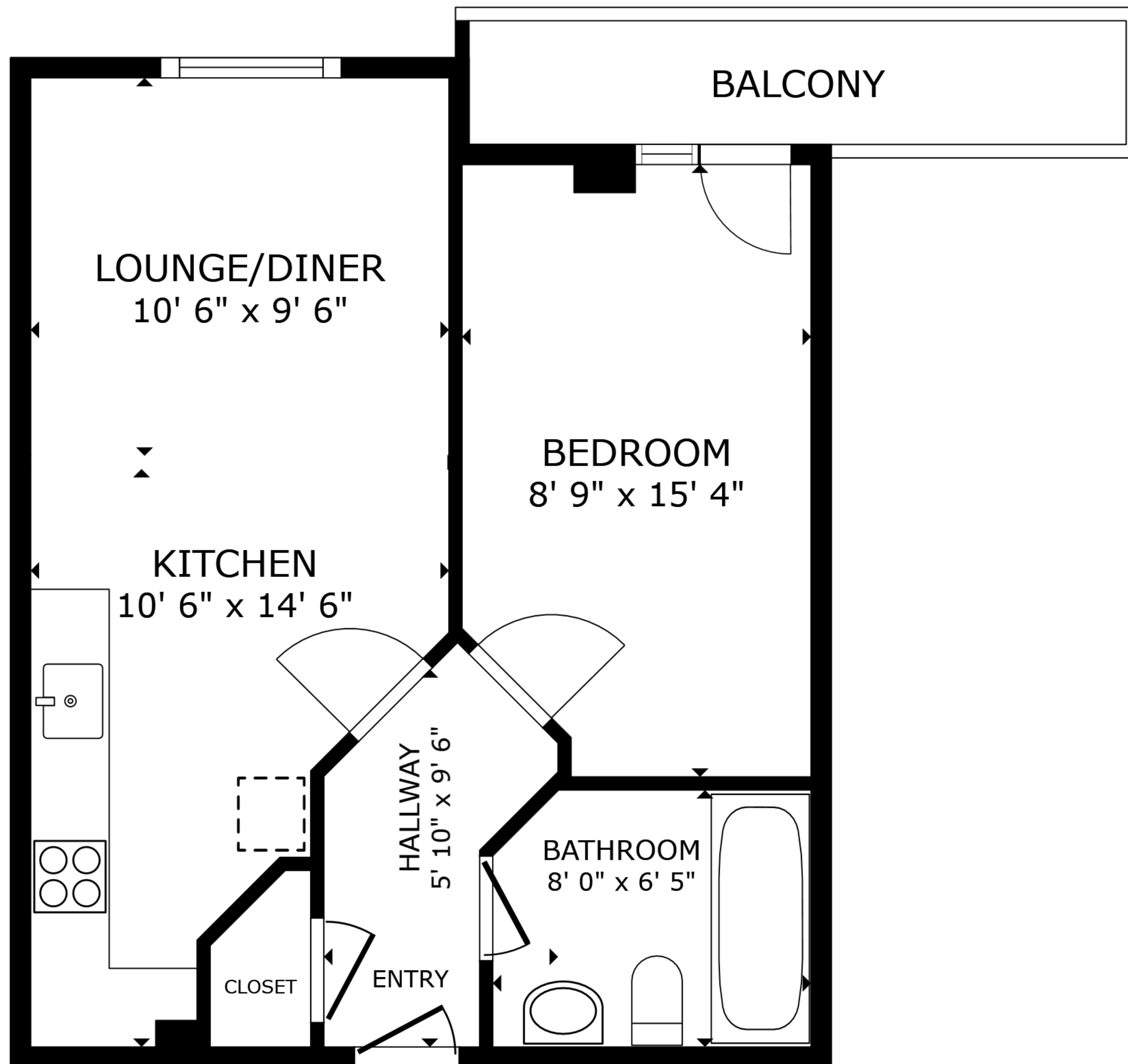
FLOOR PLAN
