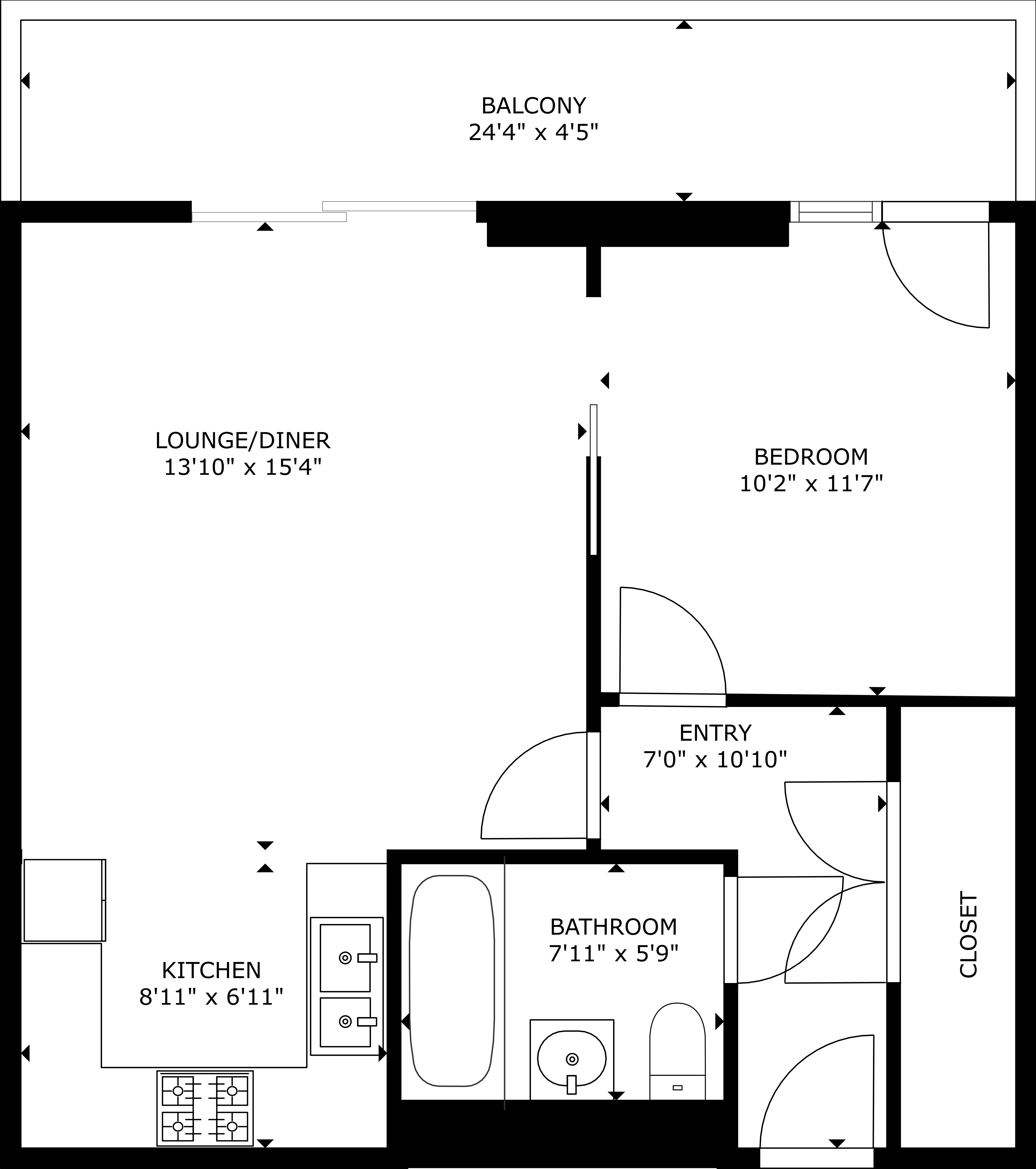
FLOOR PLAN
