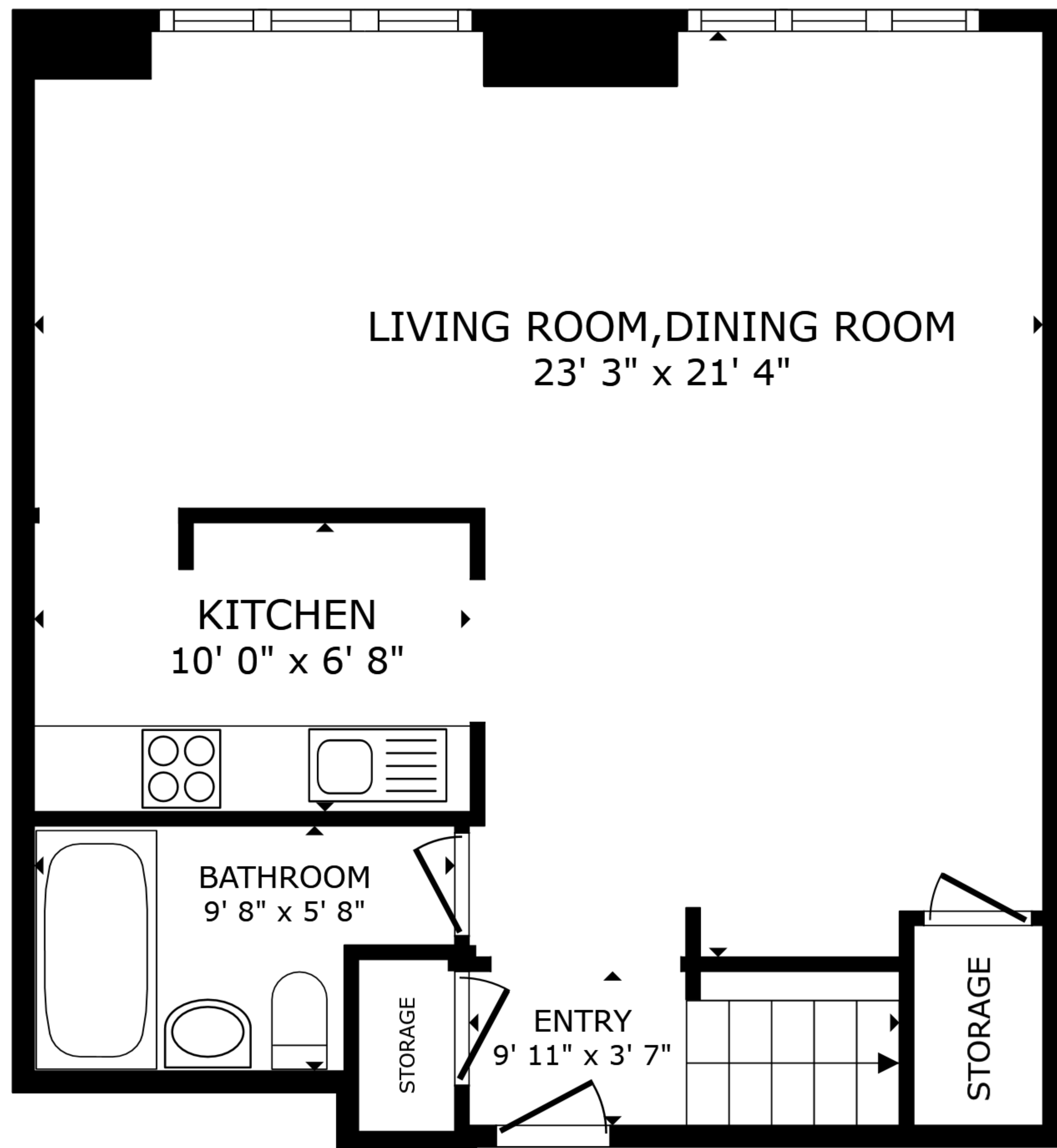
FLOOR 1
