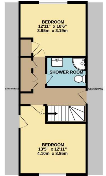
2ND FLOOR 630 sq.ft. (58.5 sq.m.) approx.
