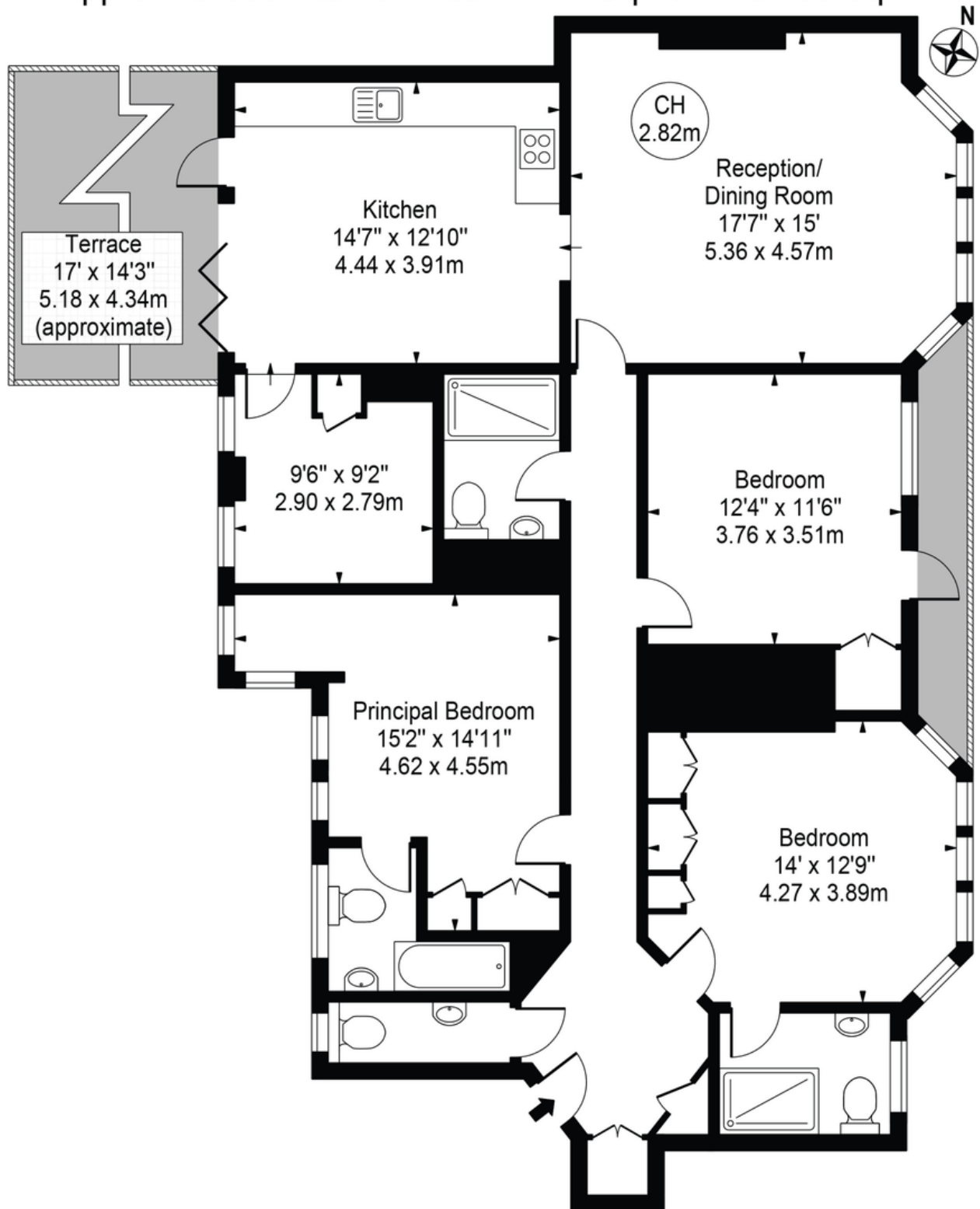
Third Floor
