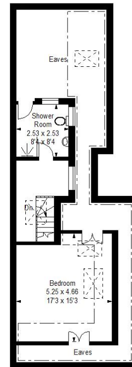
Second Floor
