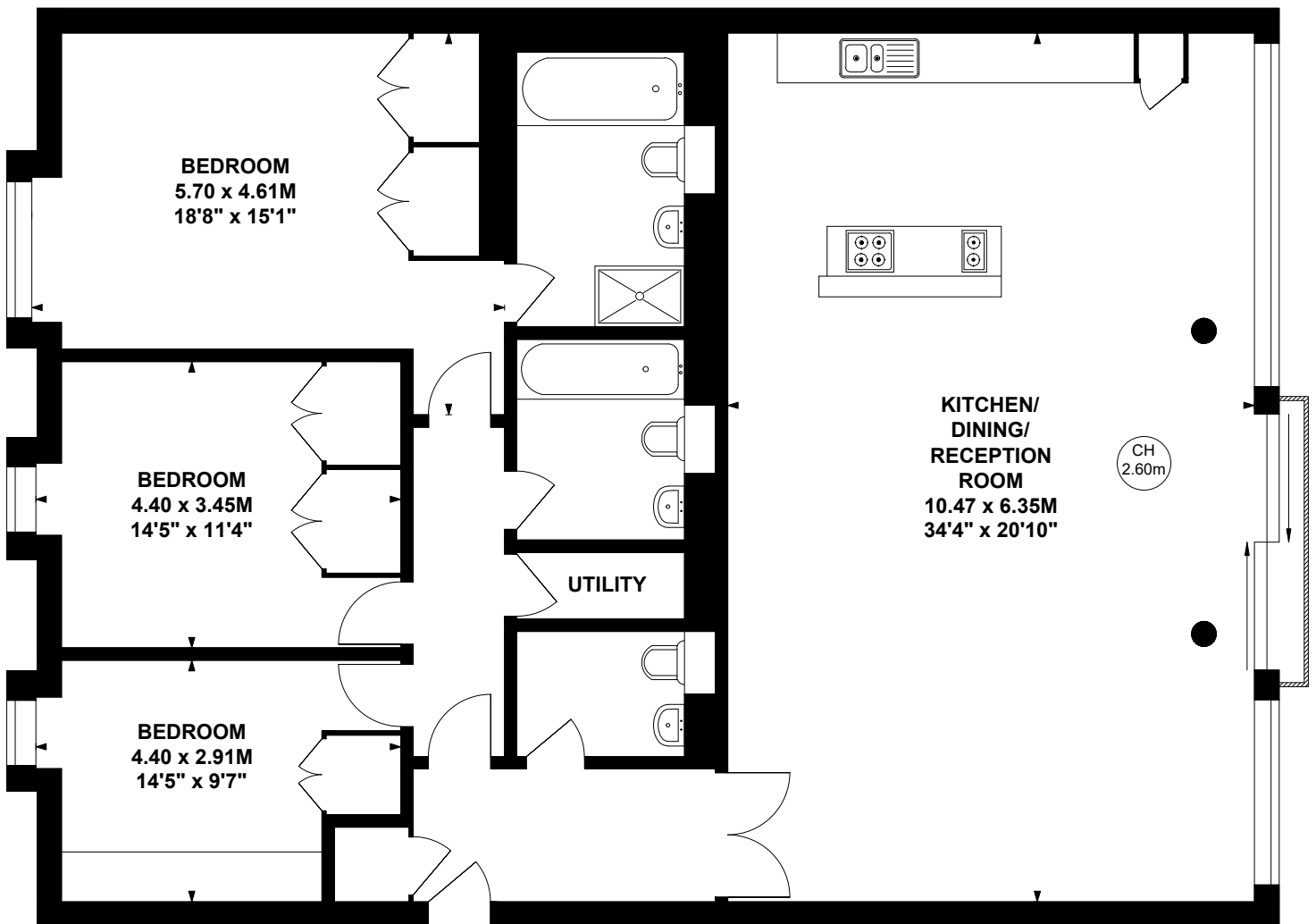
Second Floor
