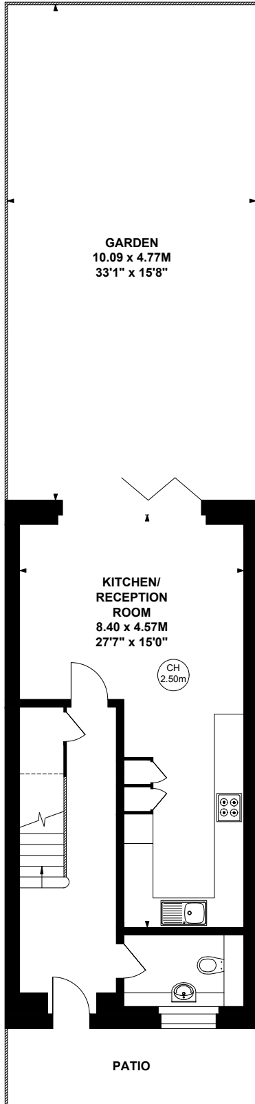
Ground Floor
