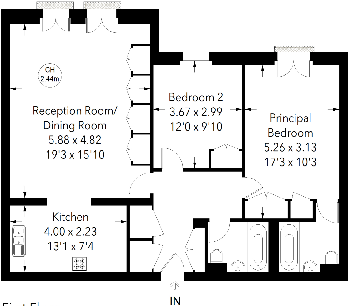
First Floor
