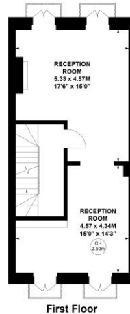
First Floor
