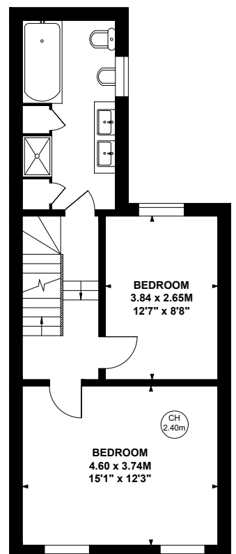
Second Floor
