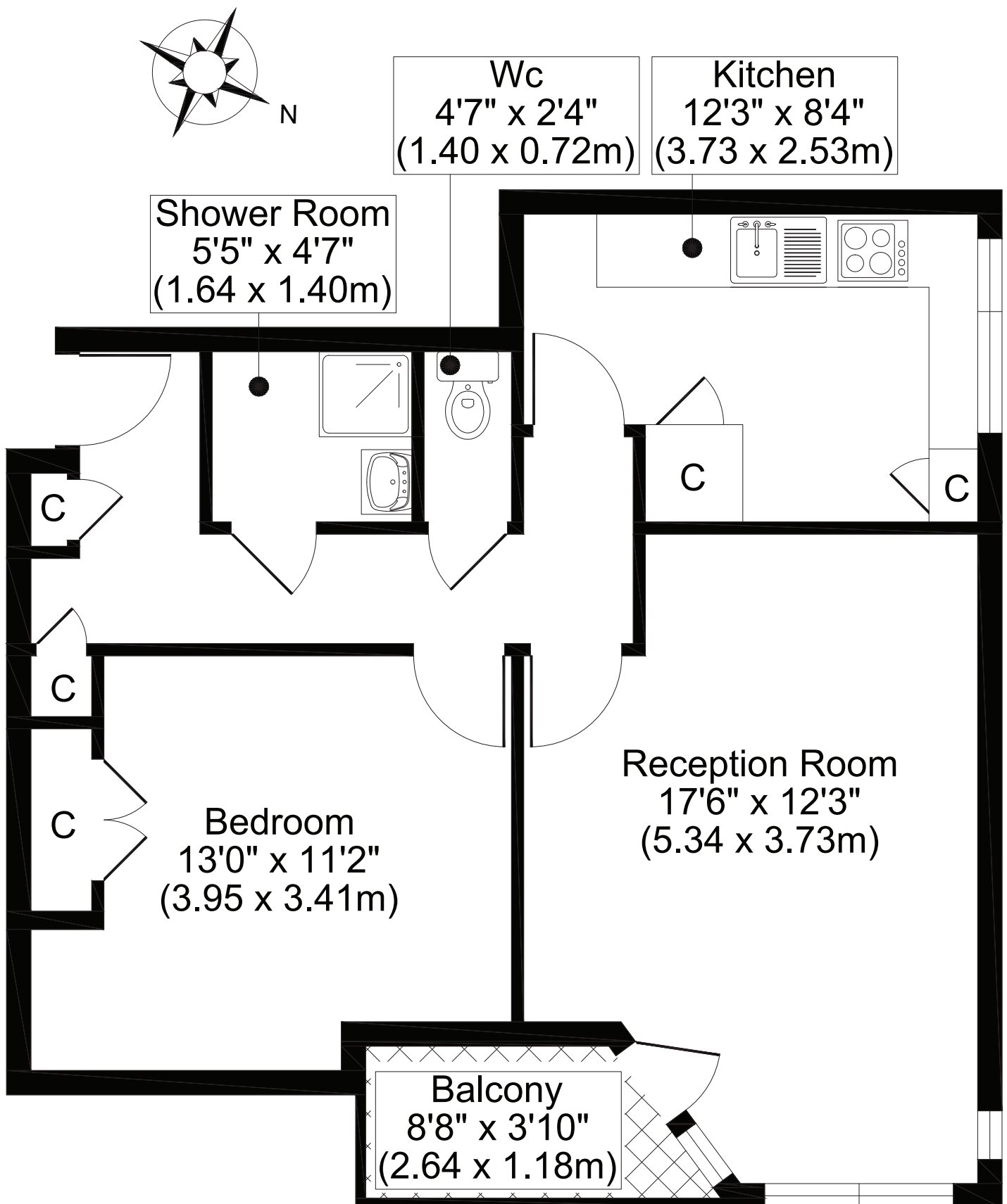
FIFTH FLOOR
