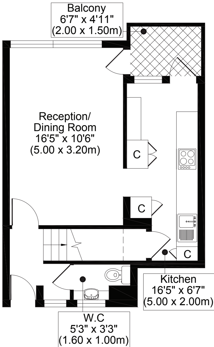
THIRD FLOOR
