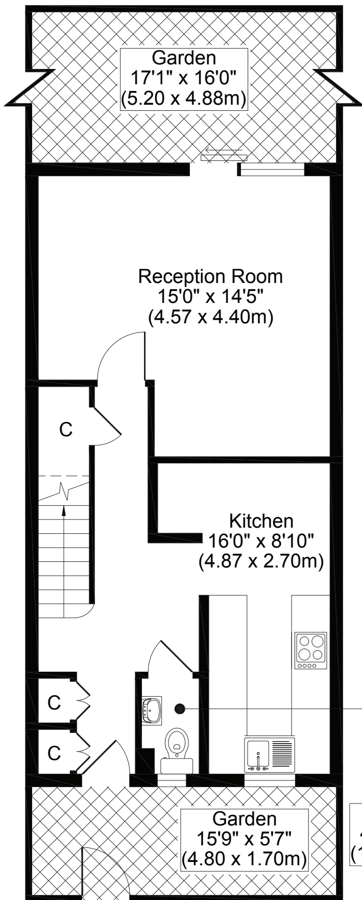
GROUND FLOOR
