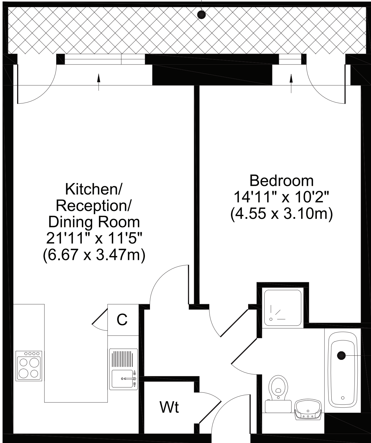
SECOND FLOOR
