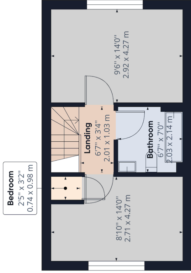
Floor 0 Building 1
