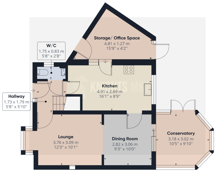
Floor 0 Building 1
