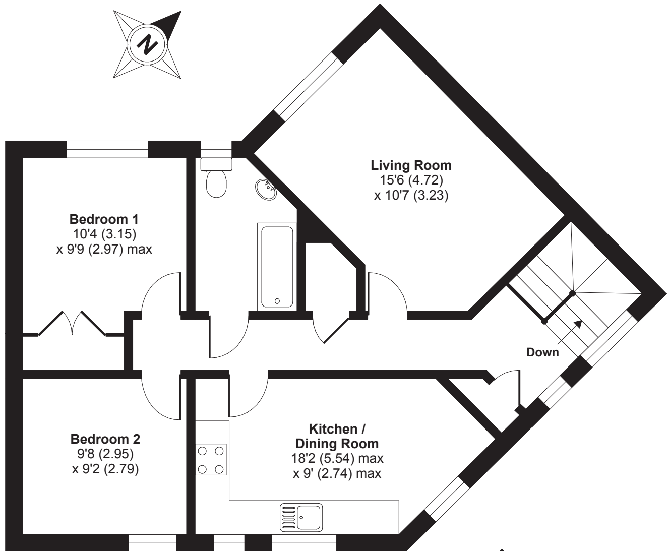
FIRST FLOOR
