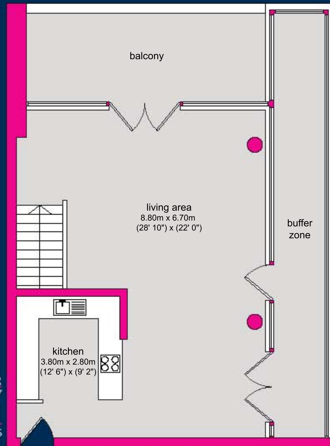
upper floor
