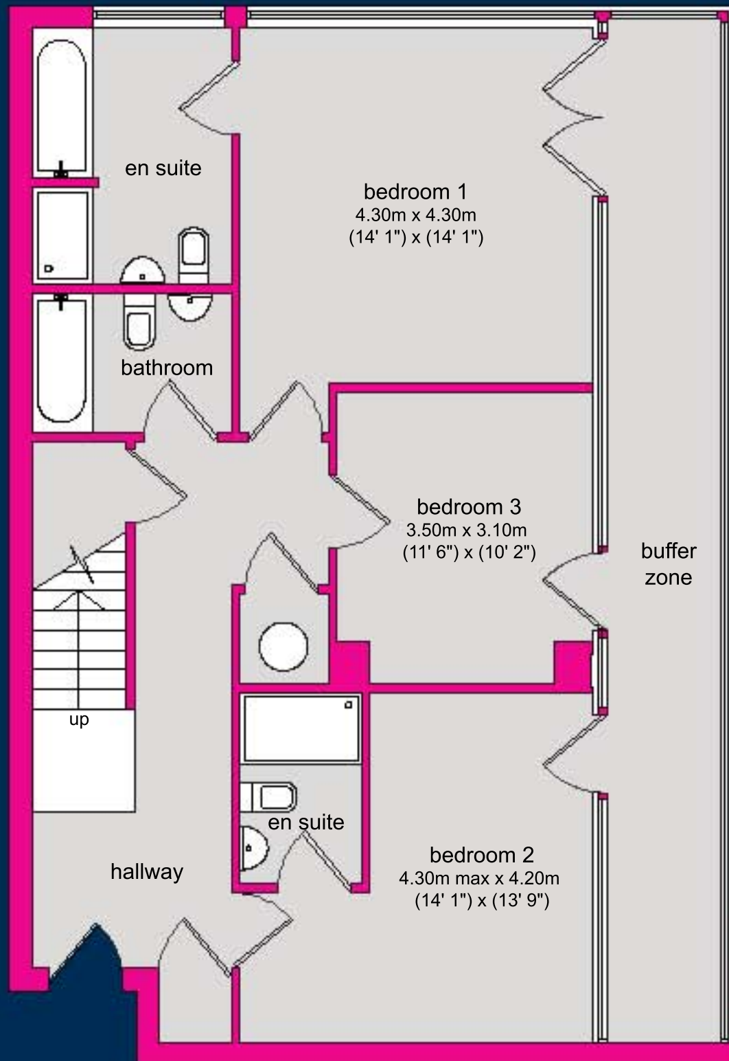
lower floor
