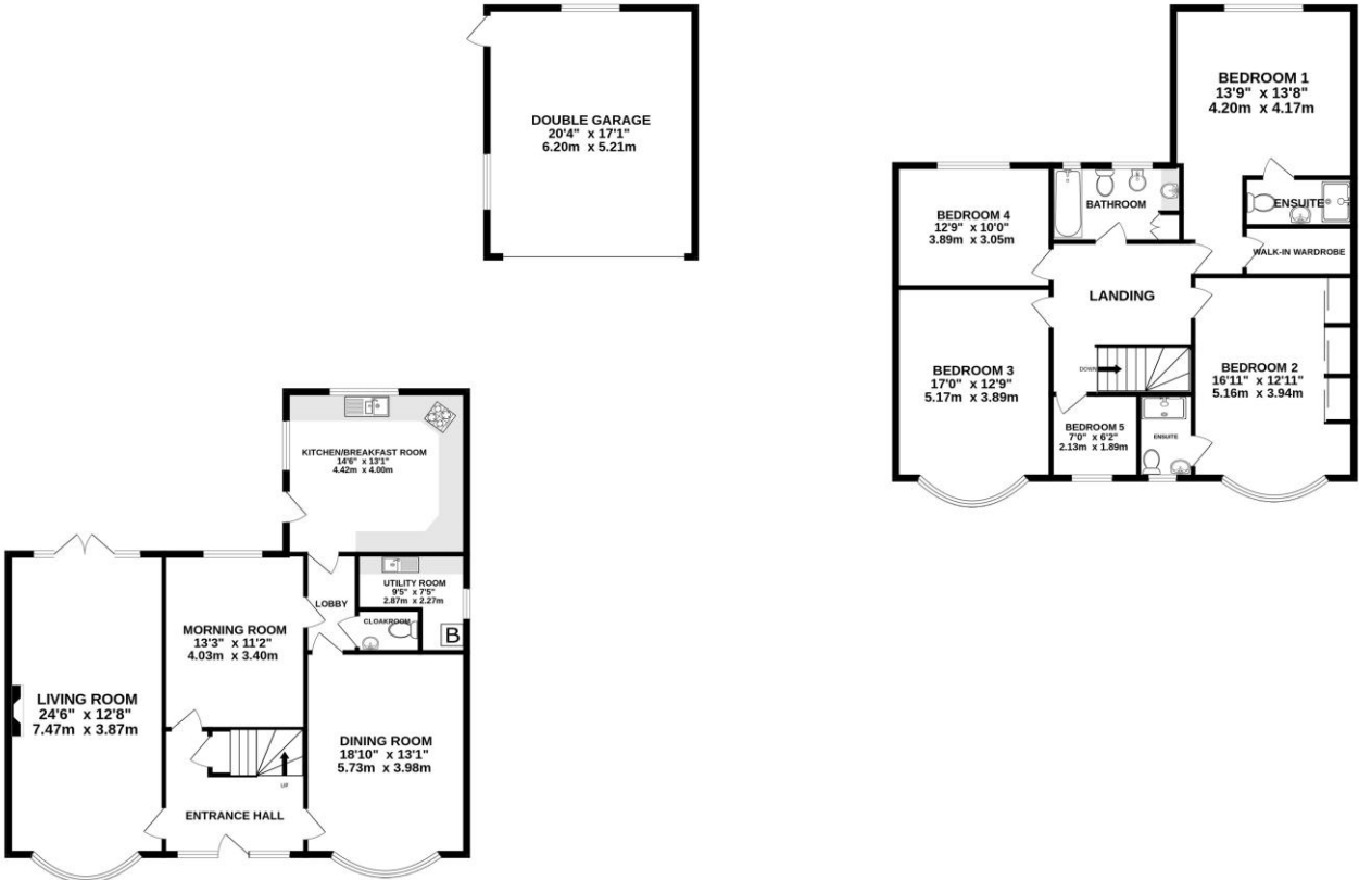
GROUND FLOOR 1475 sq.ft. (137.0 sq.m.) approx.
