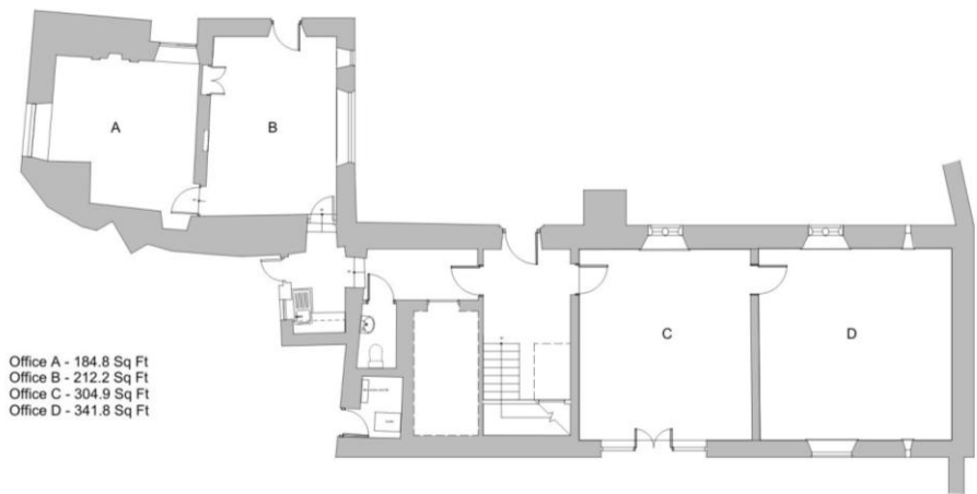
Ground Floor Scale 1:100 at A3
