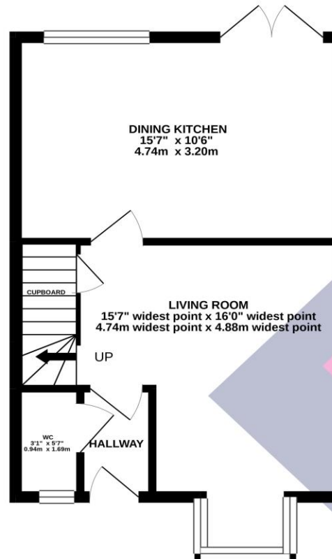
GROUND FLOOR 379 sq.ft. (35.2 sq.m.) approx.
