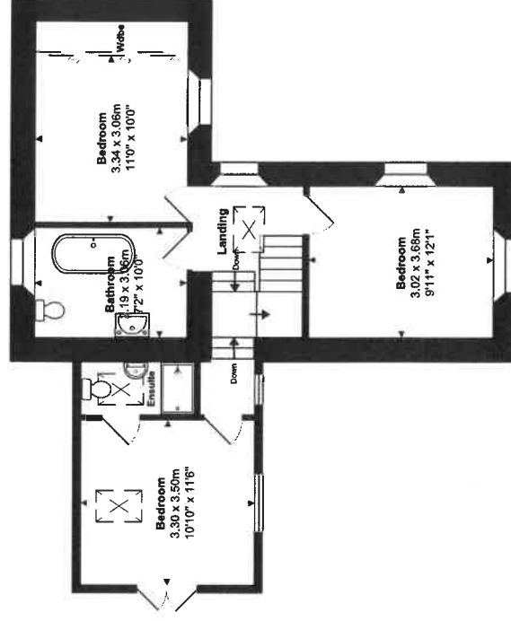
1st Floor Area (approx): 55.3 m 2 ... 595 ft 2
