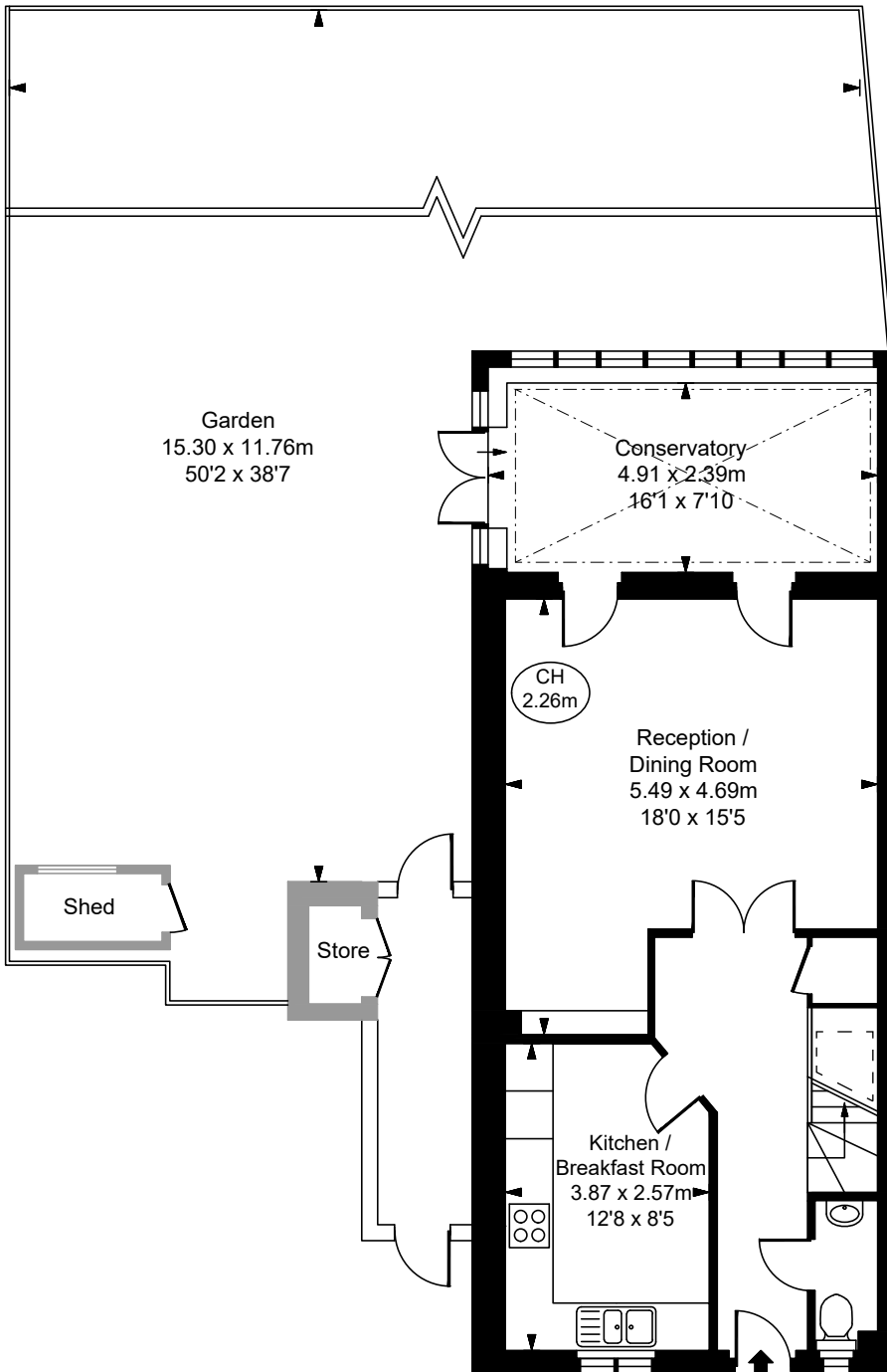
Ground Floor Approximate Gross Internal Area 57.42 sq m / 618 sq ft
