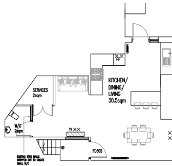
PROPOSED BASEMENT FLOOR PLAN LAYOUT 1:100 @ A2
