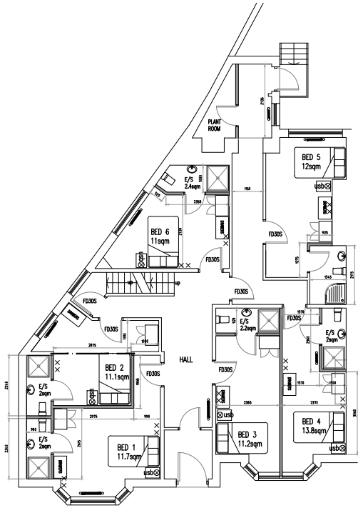
PROPOSED GROUND FLOOR PLAN LAYOUT 1:100 @ A2
