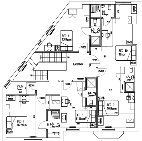
PROPOSED FIRST FLOOR PLAN LAYOUT 1:100 @ A2
