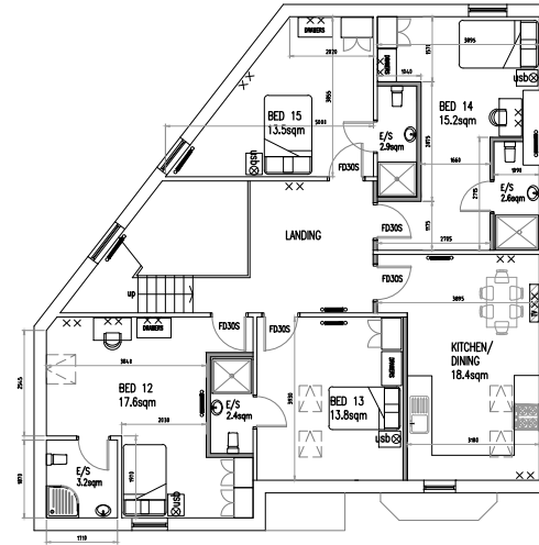
PROPOSED SECOND FLOOR PLAN LAYOUT 1:100 @ A2
