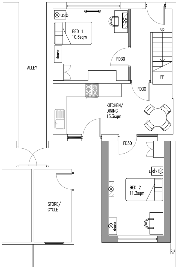
PROPOSED GROUND FLOOR LAYOUT 1:100 @ A3
