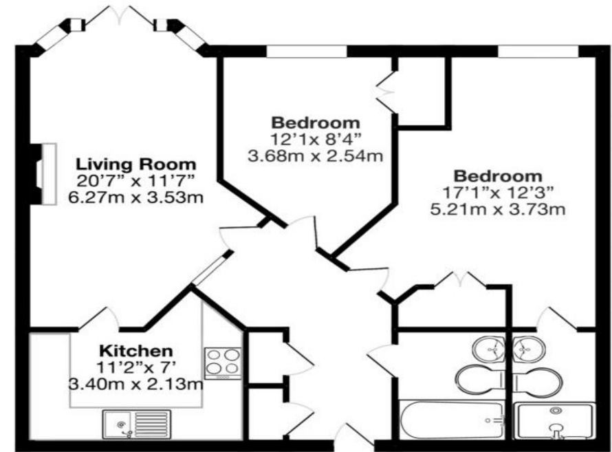
GROUND FLOOR FLAT
