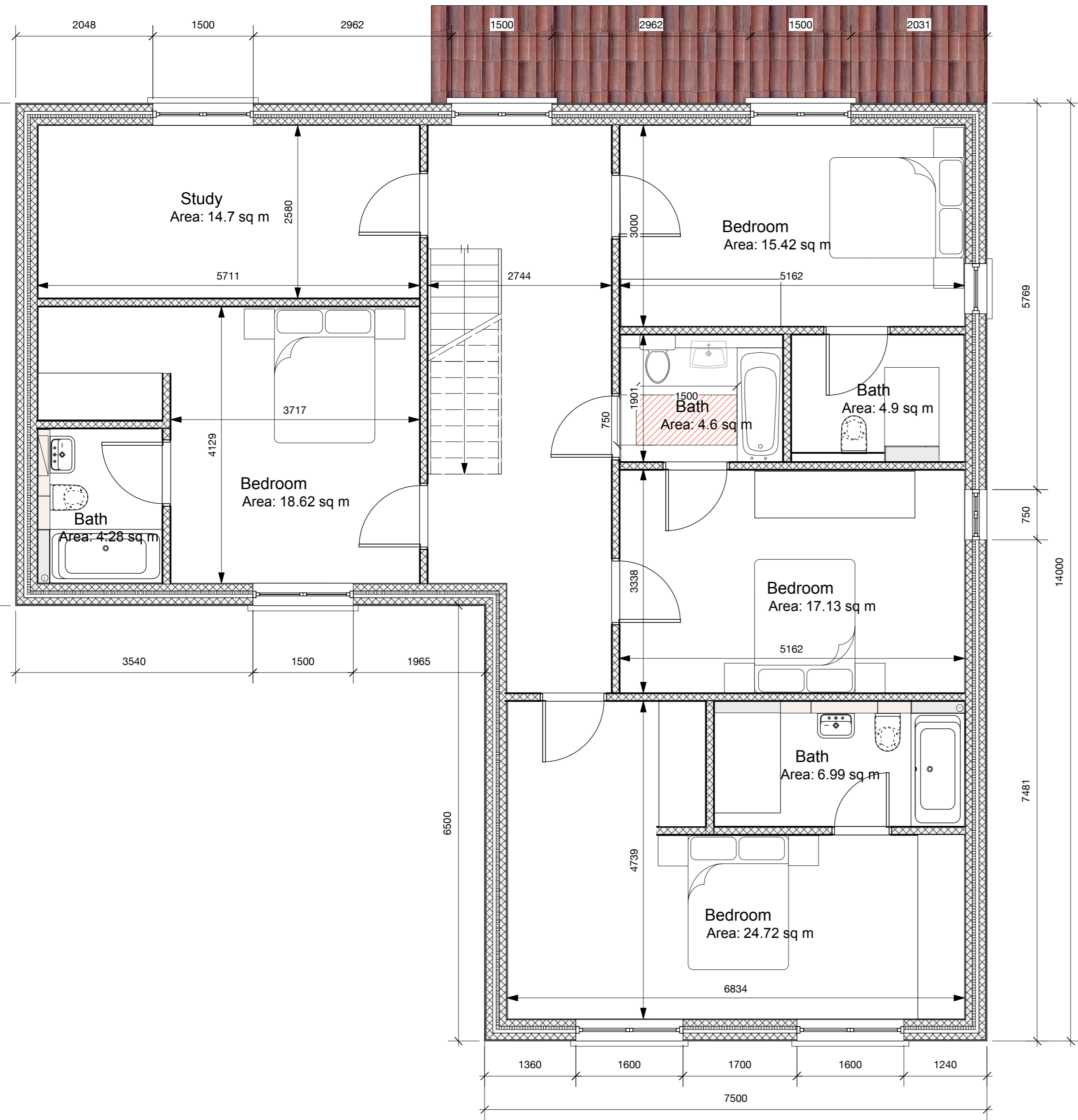
First Floor Plan - Proposed
